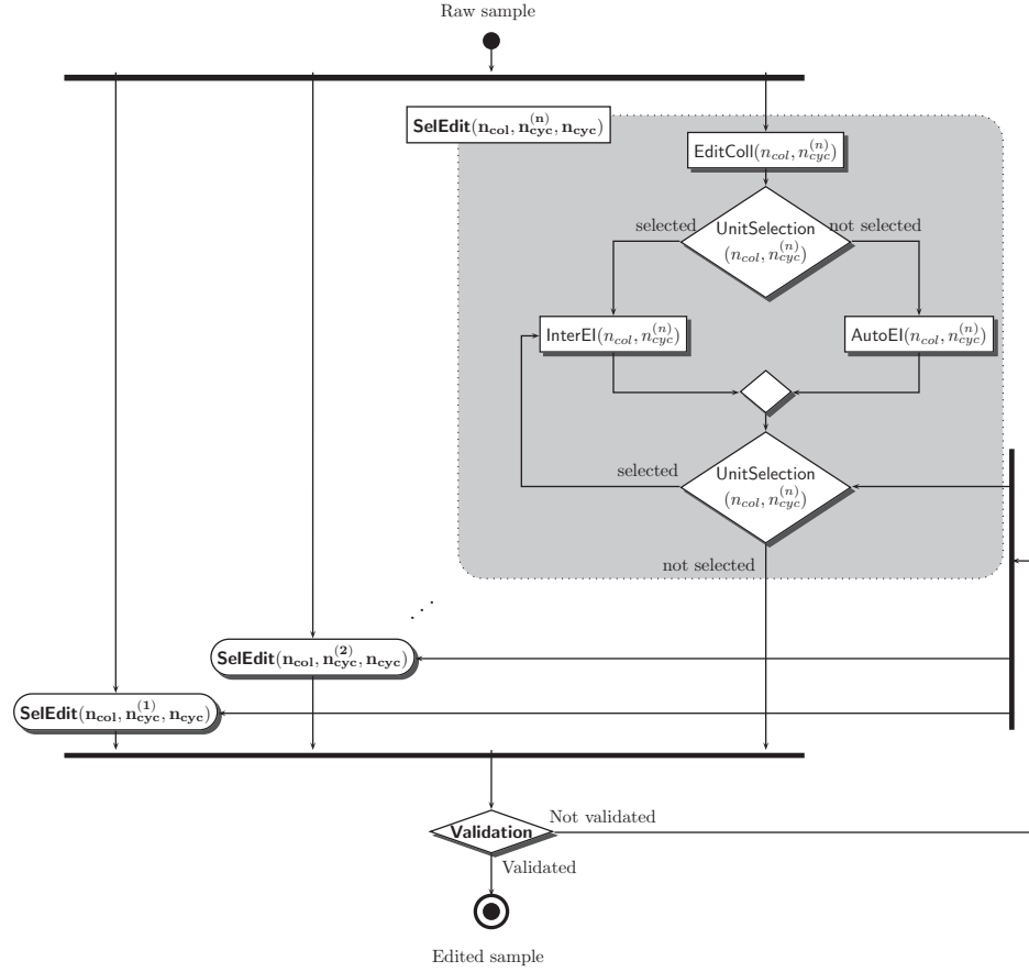
Figure 6: Extended EDIMBUS strategy workflow [71].
